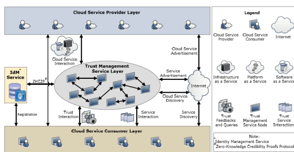
Architecture of the CloudArmor Trust Management Framework
