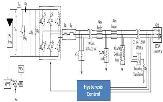
Fig 2 Circuit representation with hysteresis control.
