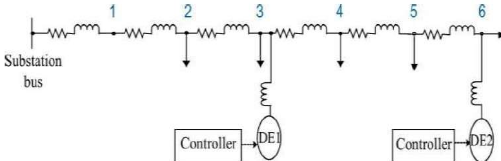
Fig 3 Base Case—A Radial Test Distribution Feeder
