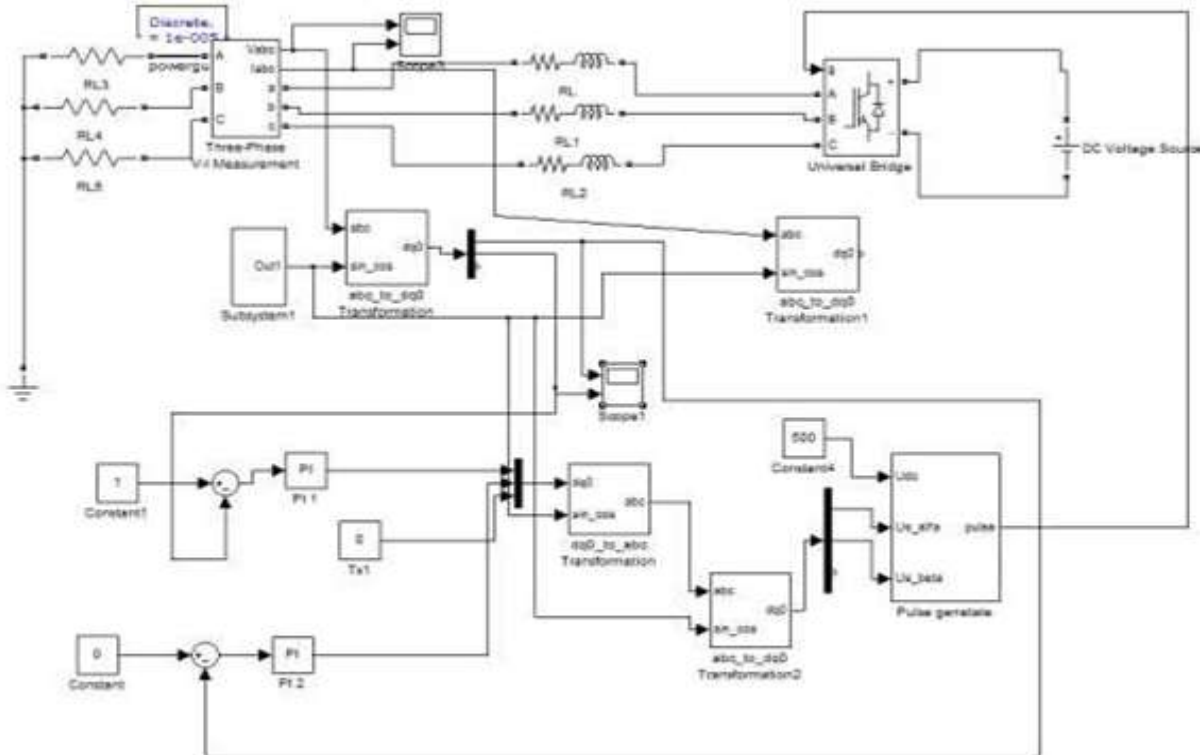
Fig 6: Simulation Diagram
