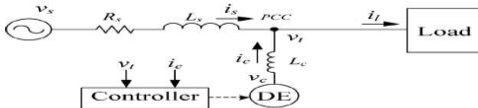
Fig 1: Parallel Connection of A DE with PE Inverter to the Distribution System
