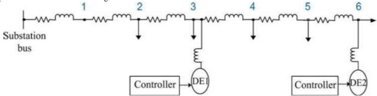
Fig 5 Base Case—A Radial Test Distribution Feeder
