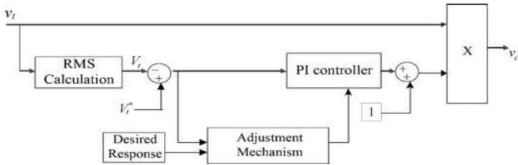
Fig. 2. Control Diagram For DE Voltage Regulation.
