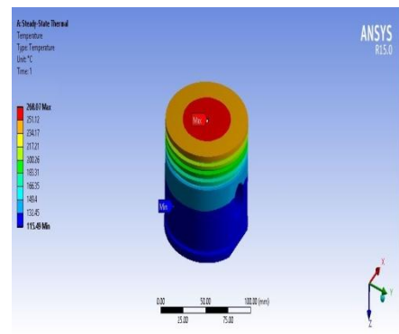
Fig 3.13: Total temperature of Al-alloy
