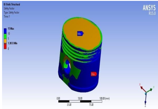
Fig 3.5: Safety factor of Steel
