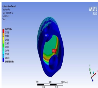
Fig 3.14: Total heat flux of Steel
