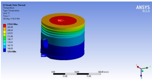
Fig 3.16: temperature of Lanthanum zirconate
