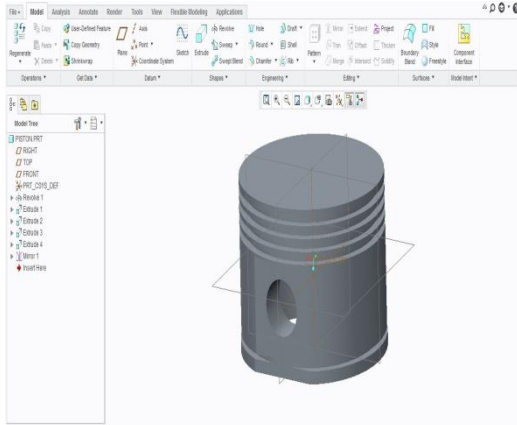
Fig 3.2: Modeled Piston
