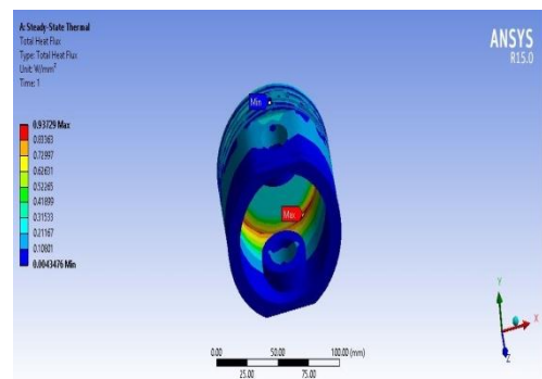
Fig 3.15: Total heat flux of Al-alloy
