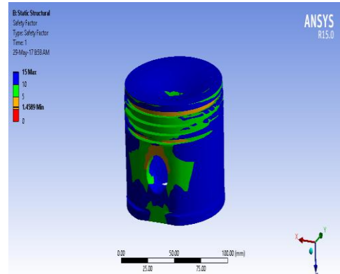
Fig 3.11: Safety factor of steel 8YSZ
