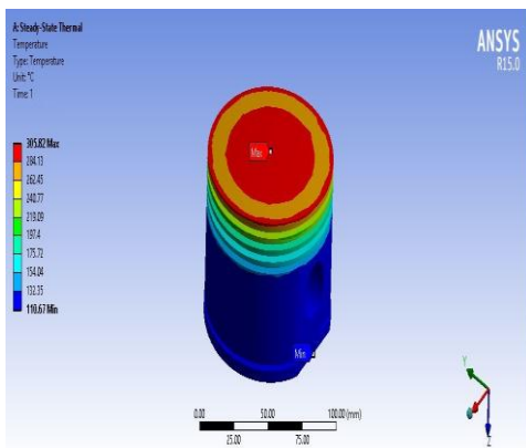
Fig 3.12: Total temperature of Steel
