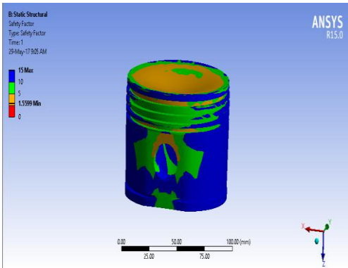
Fig 3.10: Safety factor of Lanthanum zirconate
