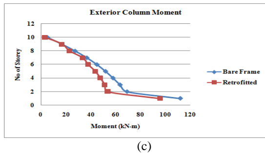
(c) Figure 7- Moment Distribution in Exterior Column of Bare Frame and Retrofitted Building for (a) Imperial Valley (b) North Ridge and (c) Loma Prieta Earthquake
