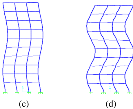
Figure 3 - Picture (a), (b), (c) and (d) represent first, second, third and fourth mode shape in X and Y directions.
