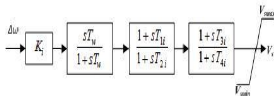
Fig 2. Structure of PSS [10]
