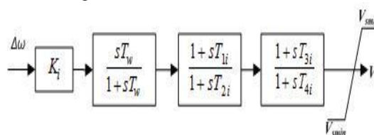
Fig 2. Structure of PSS [10]
