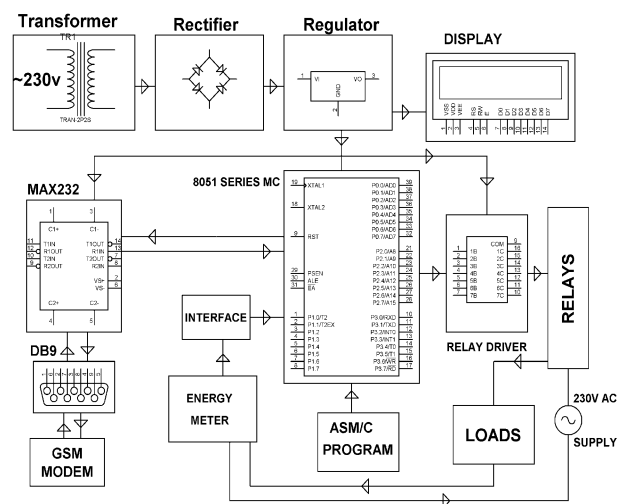
Figure 1: Block diagram of industry process automation using programmable switching GSM
