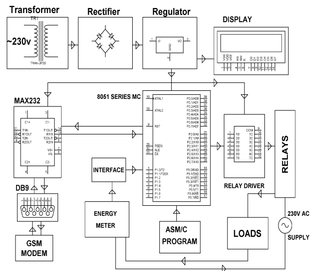
Figure 1: Block diagram of industry process automation using programmable switching GSM
