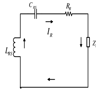
Figure .3 Equivalent circuits for Figure .2
