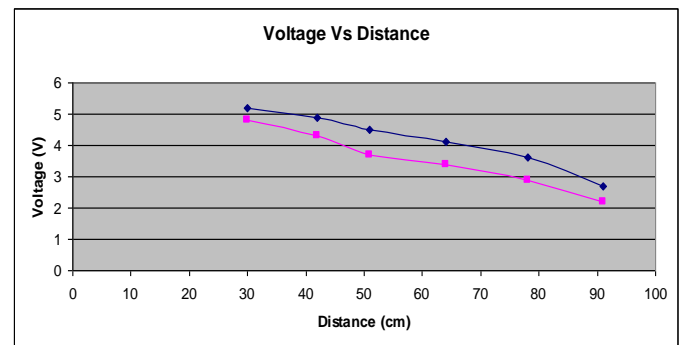
Figure.9 Theoretical and practical comparison for LED (with intermediate coil)
