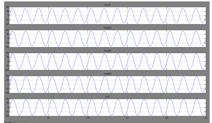
Fig.6. During a single DG unit islandingoperation harmonic voltage amplification (without damping) [from upper to lower: (a) PCC voltage (THD =4.03%); (b) node 1 voltage (THD = 3.87%); (c) node 3 voltage (THD =3.95%); (d) node 5 voltage (THD = 3.17%); and (e) DG unit filter capacitor voltage (THD = 4.65%)].
