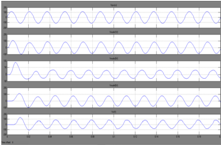
Fig.7. During a single DG unit islandingoperation harmonic voltage amplification (without damping) [from upper to lower:
