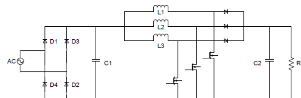
Fig. 3. Model of DC-DC interleaved Boost Converter
