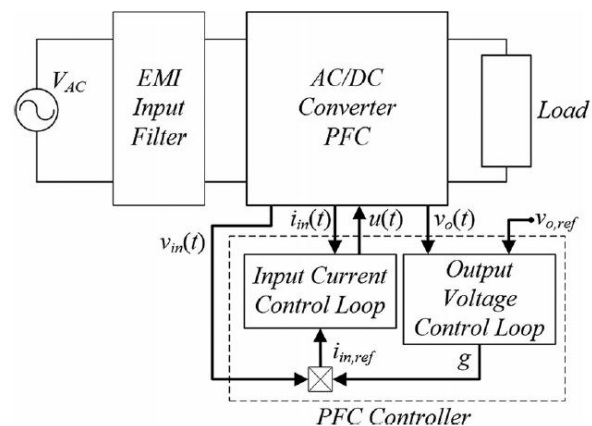
Fig. 1. Block diagram of a two-loop control for a single-phase PFC, AC to DC Rectifier.
