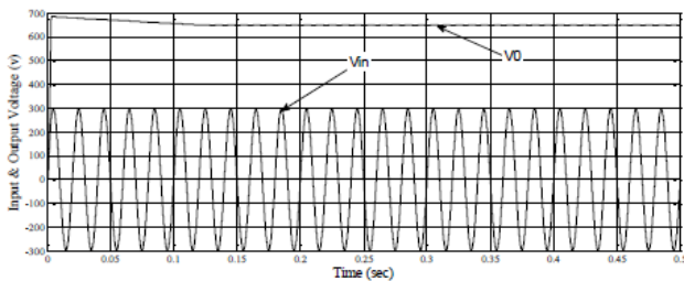
Fig. 9. Simulation waveform of output voltage for change in input voltage Fig. 9 shows clearly as change input voltage output voltage does not change for same resistive load.
