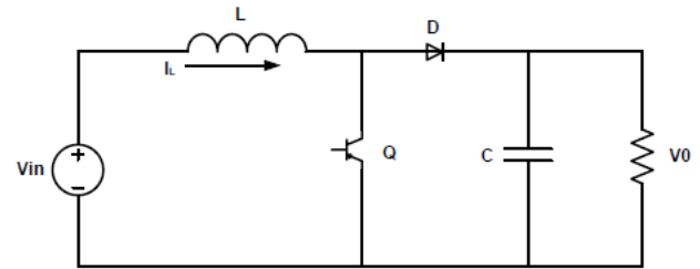
Figure 2. Boost converter
