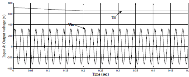
Fig. 8. Simulation waveform of output voltage for change in input voltage Fig. 8 shows waveform of output voltage which remains unchanged as input voltage change of interleaved dc-dc boost converter.
