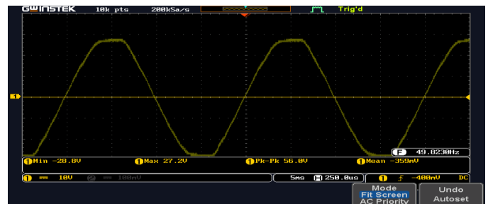
Fig. 15. Hardware Input voltage waveform
