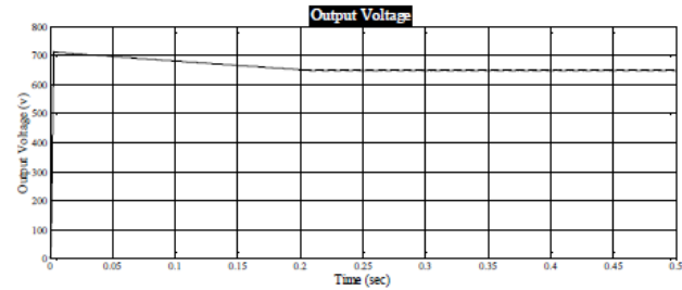
Fig. 5. Simulation waveform of output voltage
