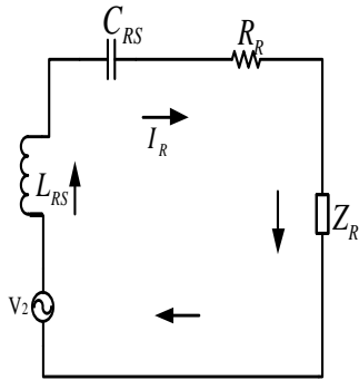
Figure.4 The equivalent circuit diagram for Figure .3 with voltage drop due to mutual impedance
