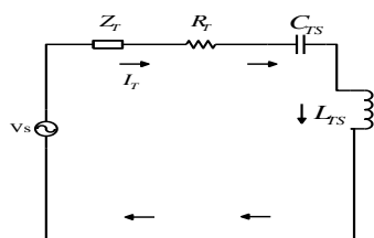
Figure.3 Equivalent circuits for theoretical model
