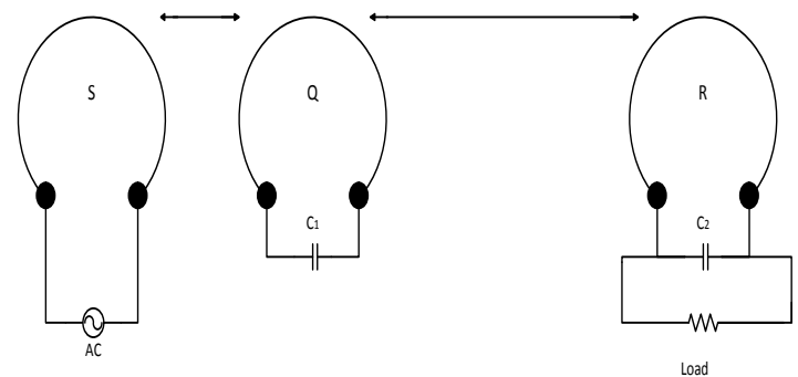
Figure.1 Theoretical Model of the System
