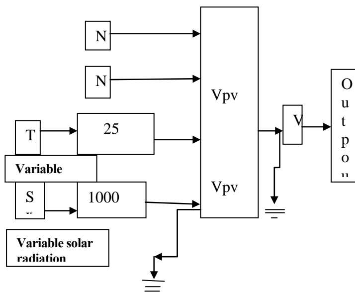
Figure1: PV Array model used in the proposed circuit
