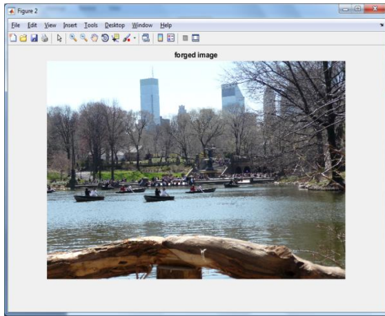
Fig 5. 2: Forged Image
