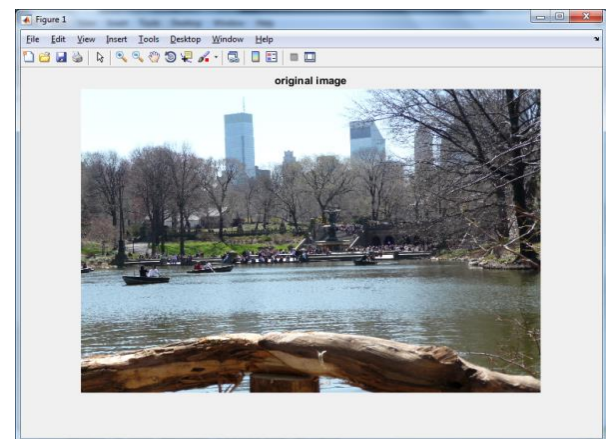
Fig 5.1: Original Image
