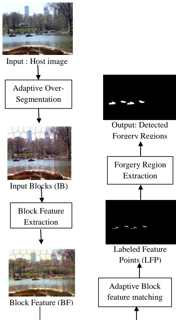
Fig.1: The proposed copy-move forgery detection scheme framework
