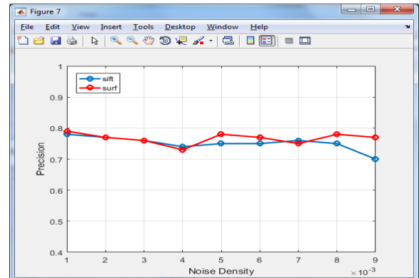
Fig 5.13 Noise Effect
