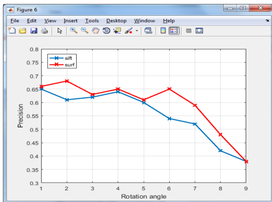
Fig 5.12 Rotation Effect
