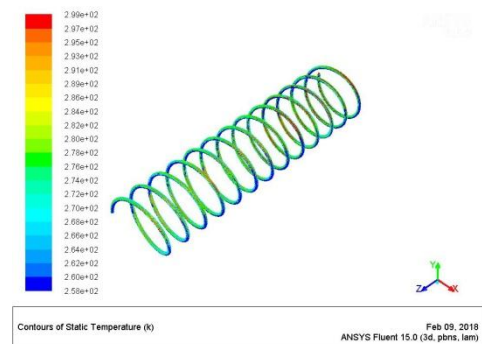
Fig 4.9: Image showing temperature analysis of aluminium helical coiled capillary tube of coil diameter 30 mm of R407C
