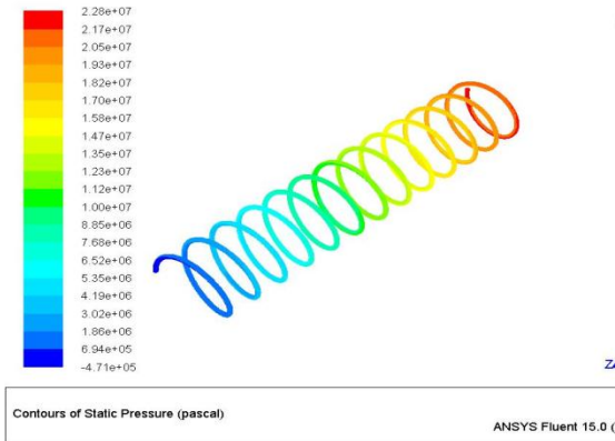
Fig 4.5: Image showing pressure analysis of aluminium helical coiled capillary tube of coil diameter 25mm of R407C
