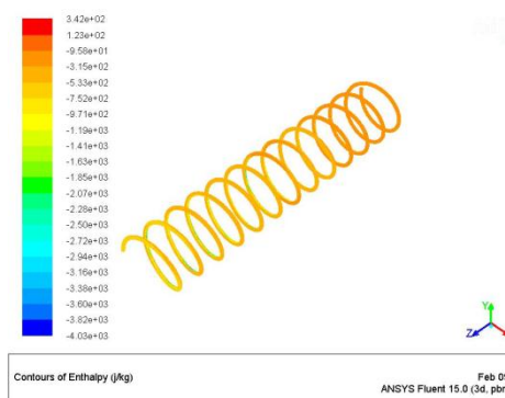
Fig 4.7: Image showing enthalpy analysis of aluminium helical coiled capillary tube of coil diameter 25mm of R407C
