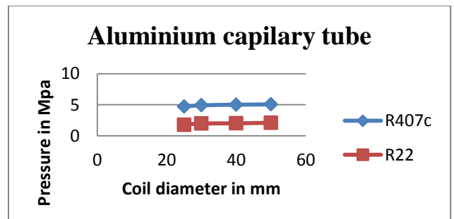
Graph: 5.1. According to this plot, pressure varies with respect to coil diameter.
