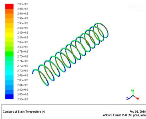
Fig 4.6: Image showing temperature analysis of aluminium helical coiled capillary tube of coil diameter 25mm of R407C
