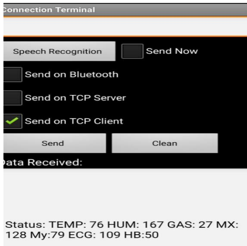
Fig.15.Data received to connection terminal through Wi-Fi in Mobile.
