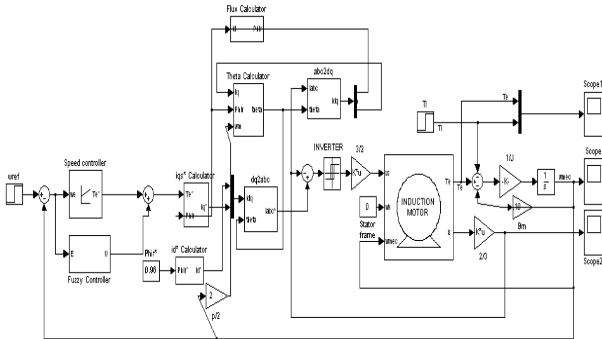
Figure 5: SIMULINK Model of Induction motor using hybrid PI -Fuzzy controller
