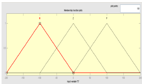
Figure 3: Membership function for Input variables
