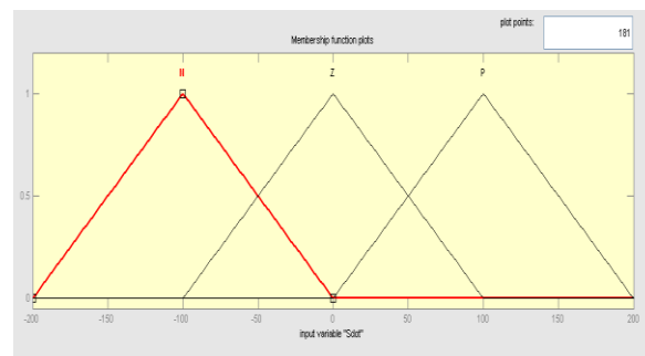
Figure 3: Membership function for Input variables
