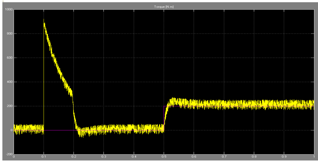
Figure 9: Torque Response of Induction Motor using hybrid PI-fuzzy Control.
