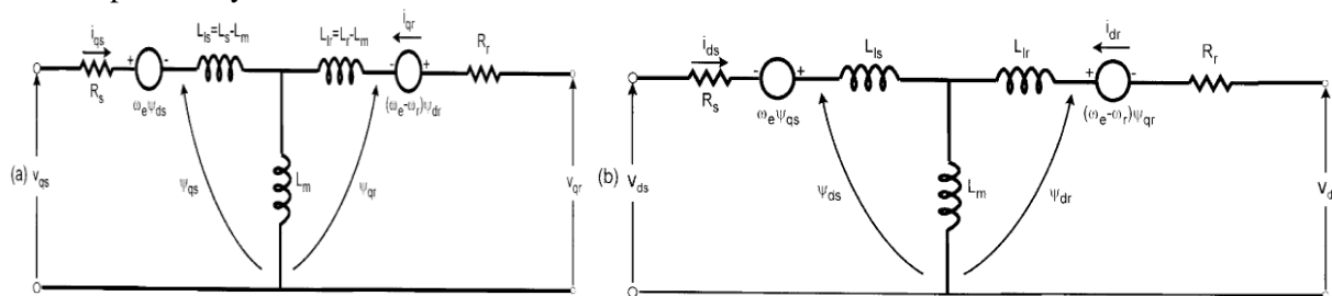
Figure 1: Stator and rotor in two-axis reference frame (a) q-axis, and (b) d-axis
