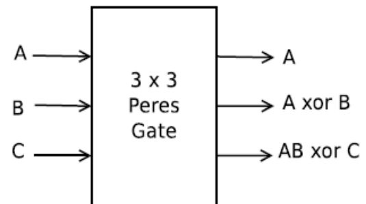
Fig. 6: Peres Gate
