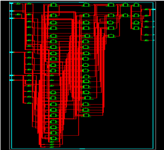
Fig. 15: Technology schematic of Reversible 4X5 TCAM Array
