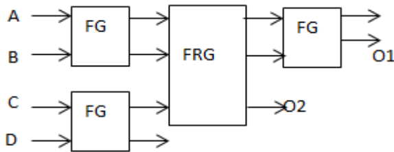
Fig.11: Proposed 4:2 Reversible Encoder.
