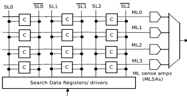
Fig. 1: Conventional 4 × 3 TCAM Array
