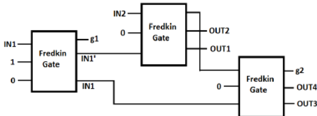
Fig. 12: Proposed reversible 2:4 decoder
