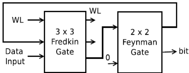
Fig. 7: SRAM Cell using Reversible Gates
