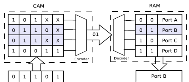
Fig. 3: Application of TCAM in Routing Table
