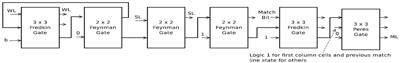
Fig. 9: Reversible TCAM Cell
