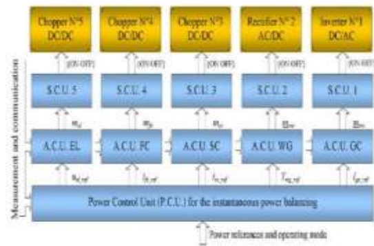
Fig.3.Hierarchical control structure of the HPS
