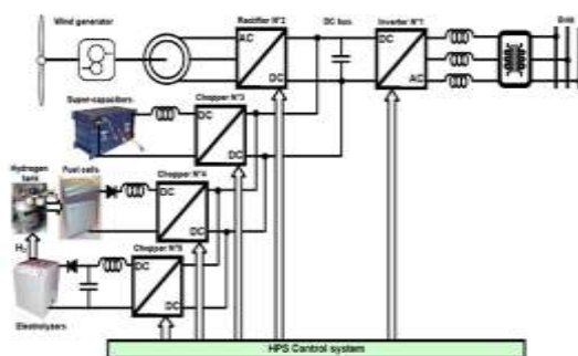
Fig 2. Structure of the studied wind/hydrogen/SCHPS
