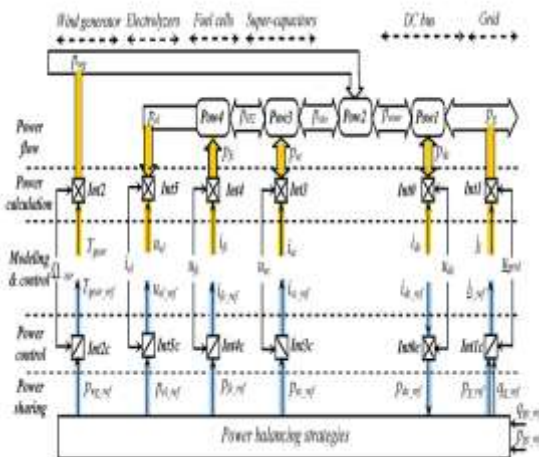
Fig 5 Multilevel representation of the power modeling and control of the HPS
