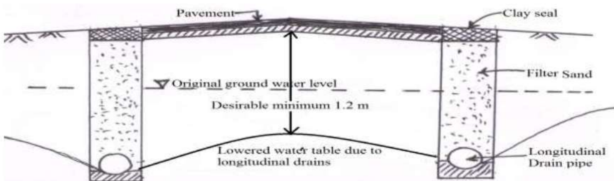
Lowering High Water Table in Permeable Soils
