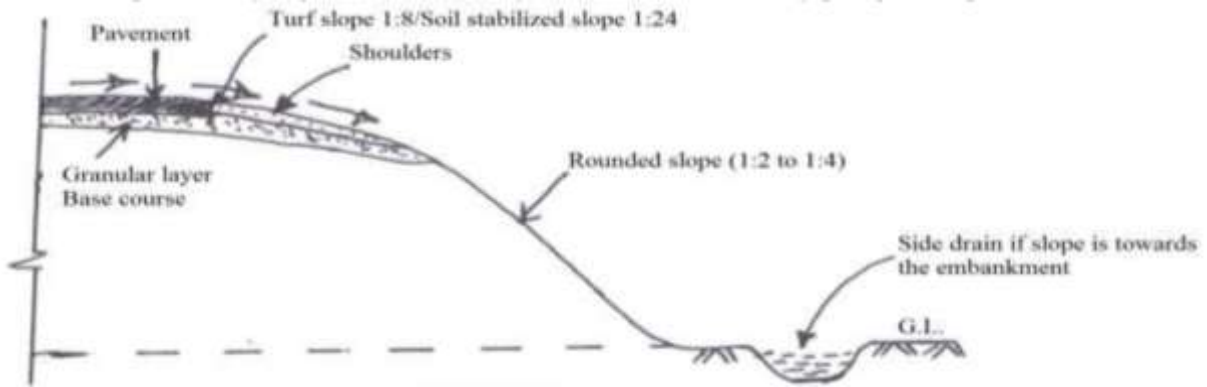
Surface Drainage in Road embankment
