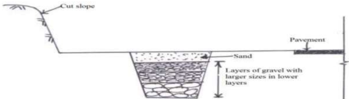
Surface Drainage in Cutting
