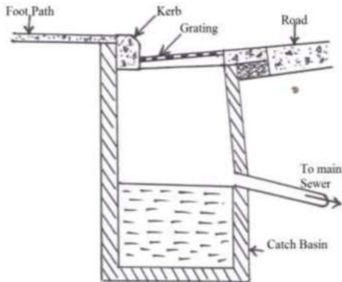
Cross Section of Grating Catch Basin
