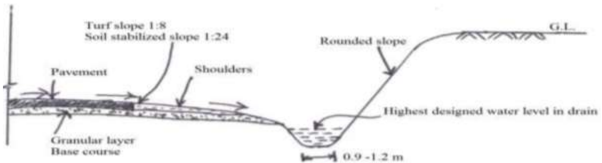
Surface Drainage in Cutting
