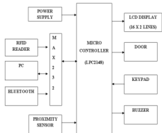
Fig1: Tracking section
