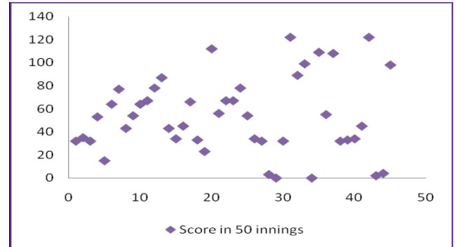
Fig 16: Scatter Plot
