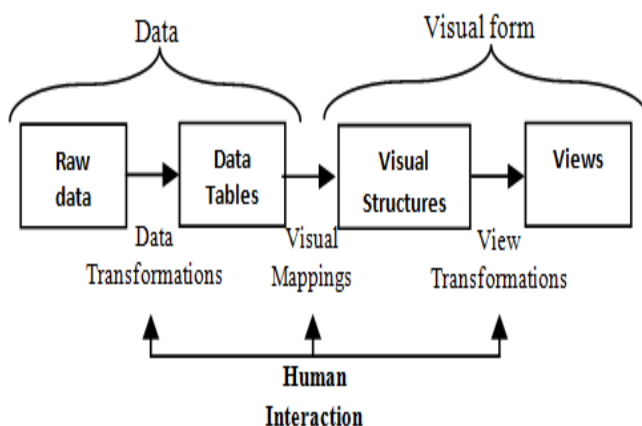
Fig 28: Interactive Mechanism
