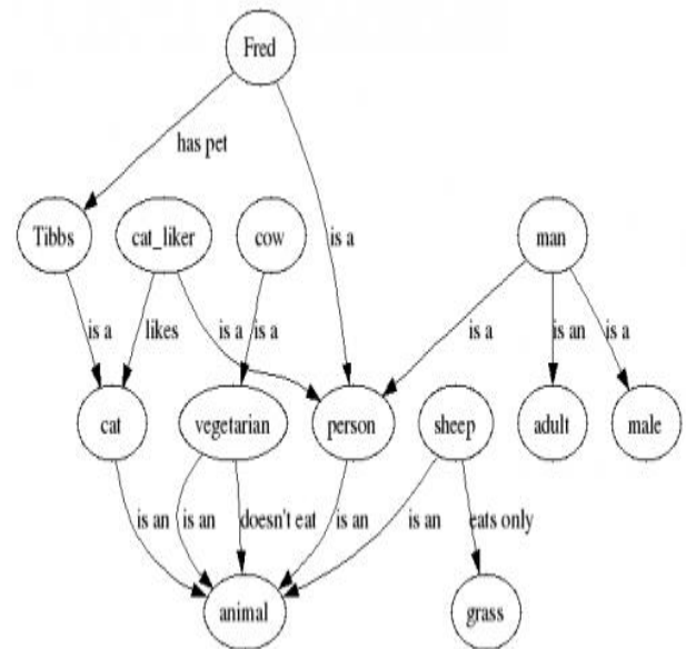
Fig 27: Semantic Network
