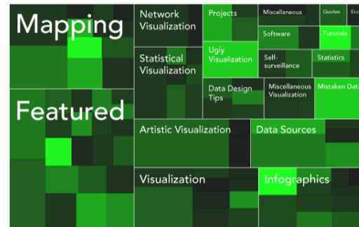
Fig 21: Tree Map
