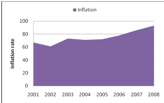
Fig 14: Area Chart
