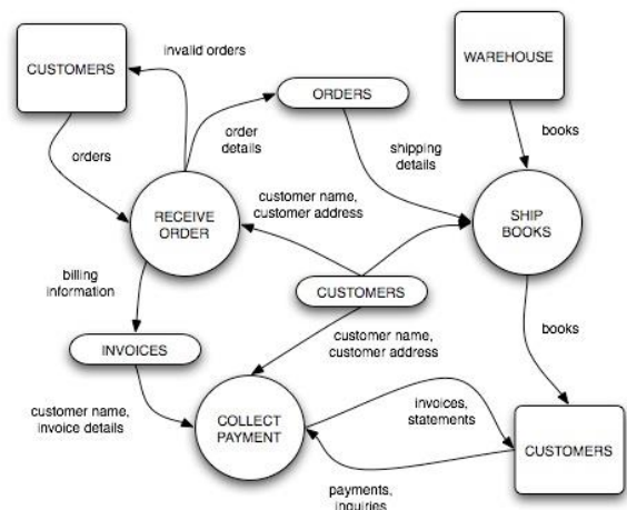
Fig 25: Data Flow Diagram
