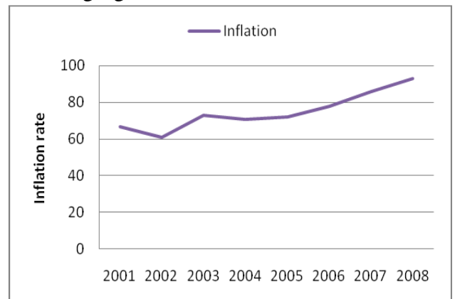
Fig 13: Line Graph
