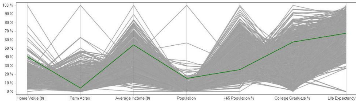
Fig 20: Parallel Coordinates
