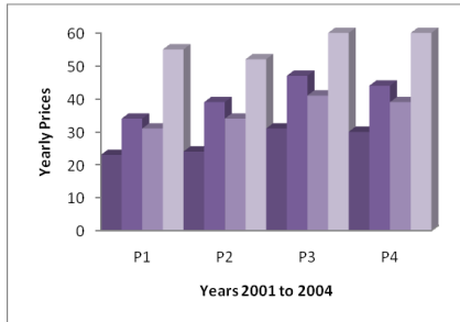
Fig 10: Histogram
