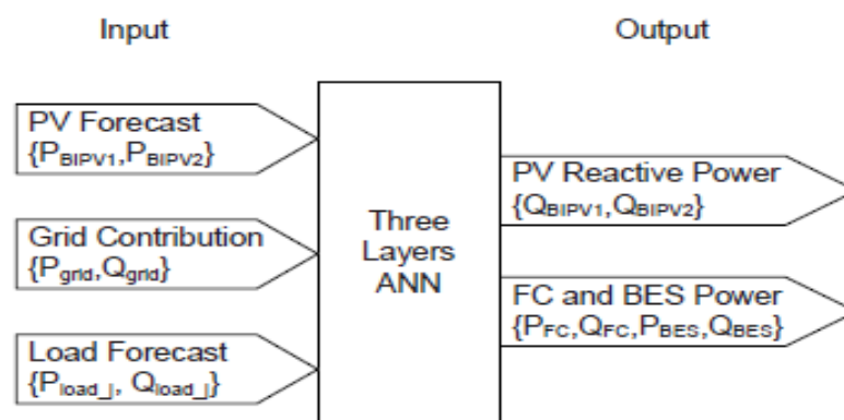
Figure 4. Microgrid controller input and output
