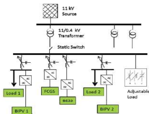
Figure 2. Proposed Microgrid architecture
