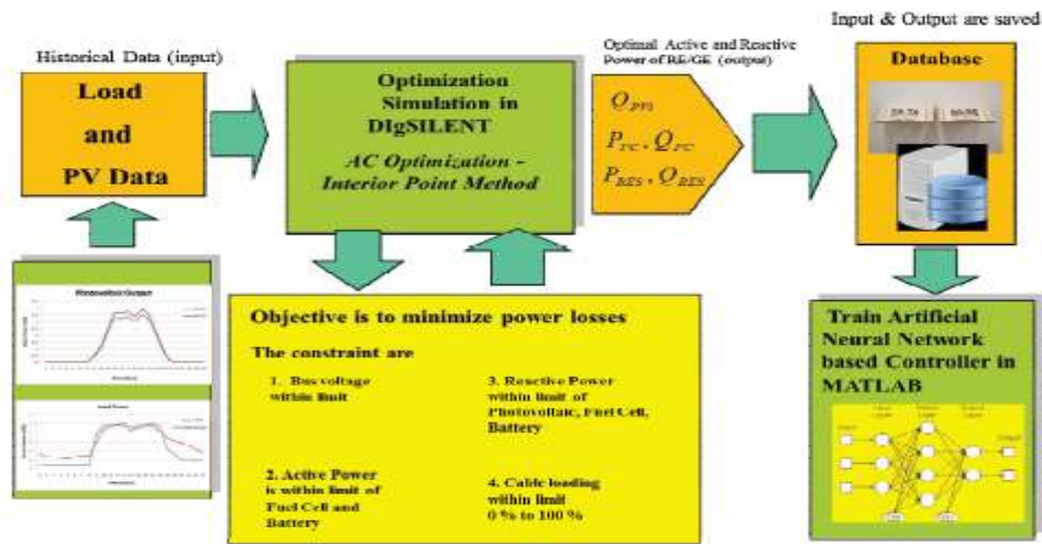
Figure 3. Microgrid controller development process
