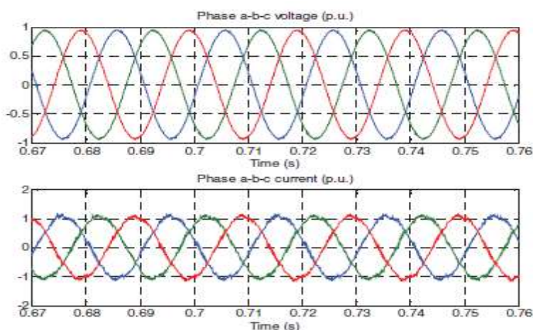
Figure 8. BESS output voltage and current
