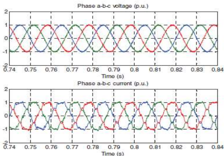
Figure 7. FCGS output voltage and current
