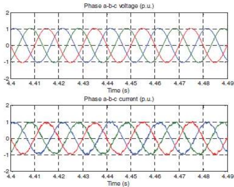
Figure 6. PVGS output voltage and current
