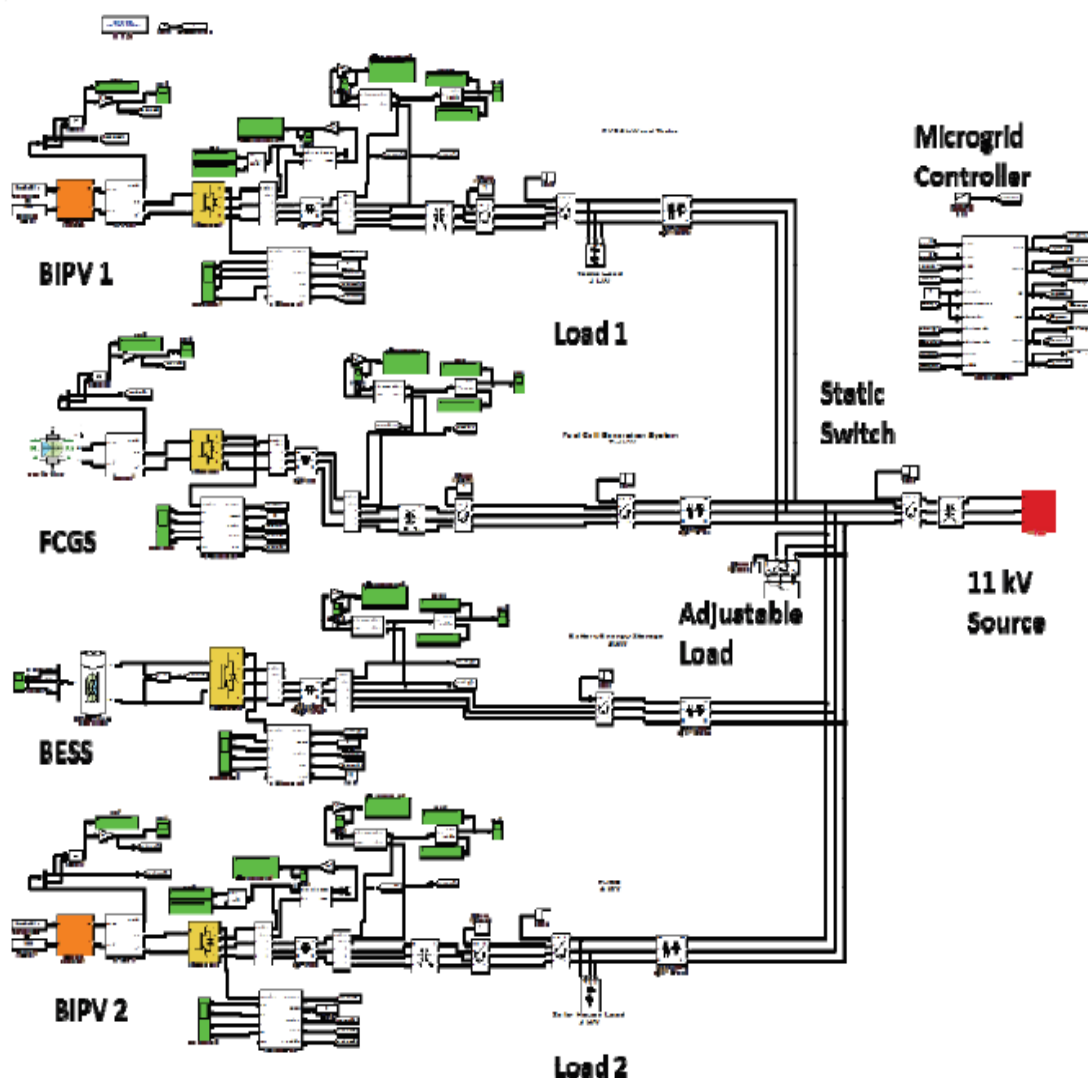
Figure 5. Snapshot of Microgrid model in SimPowerSystems
