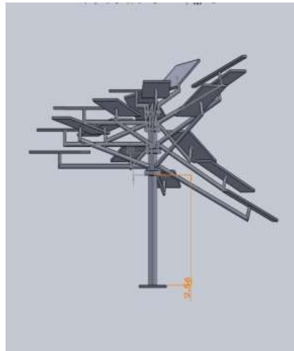
Figure 4: Side View of Proposed Solar Tree
