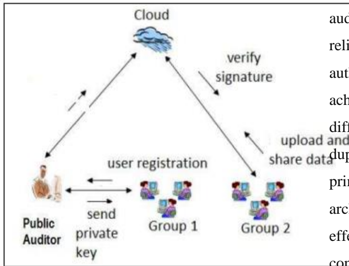
Fig. 4. Cipher Text Model
