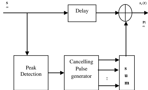
A Block Diagram of PC Implementation Using Hardware
