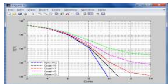
SNR vs. SER for the extension (SUI channel model).
