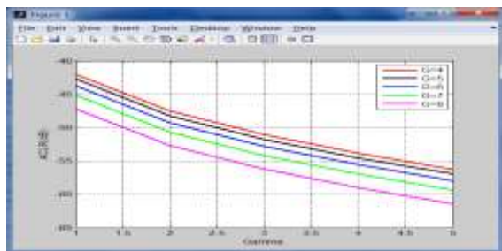
. ACLRs with respect to different pulse length n under different target PAPR \gamma
