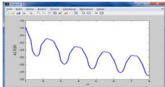
Relationship between the ACLR and the length n of a cancelling pulse kernel g(t) ; a sinc function is used as the cancelling pulse kernel.
