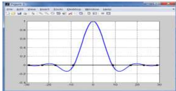
A cancelling pulse kernel considered for the proposed work is generated for the given oversampling rate J = 4 . The black dots show that the special cases of the n having integer values.
