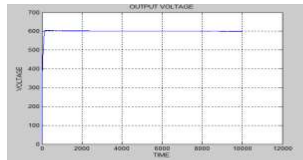
Fuzzy logic controller output voltage
