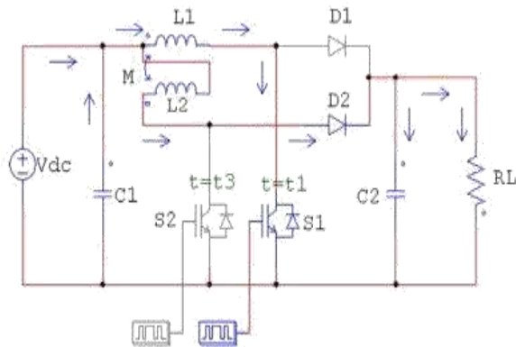
Mode 2 Circuit Diagram
