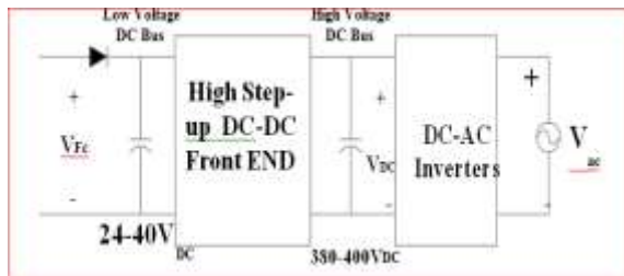
General Power generation system with a high step-up converter
