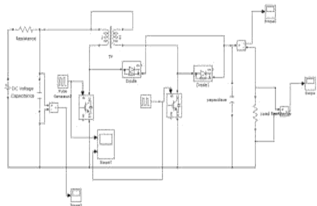
Mat lab/simulink model in open loop method
