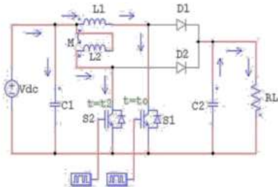
Mode 1 circuit diagram
