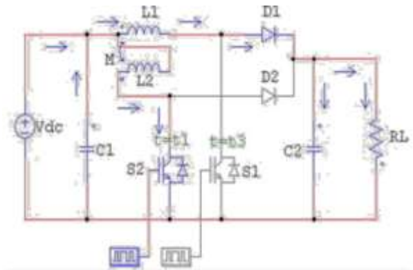
Mode 4 circuit diagram
