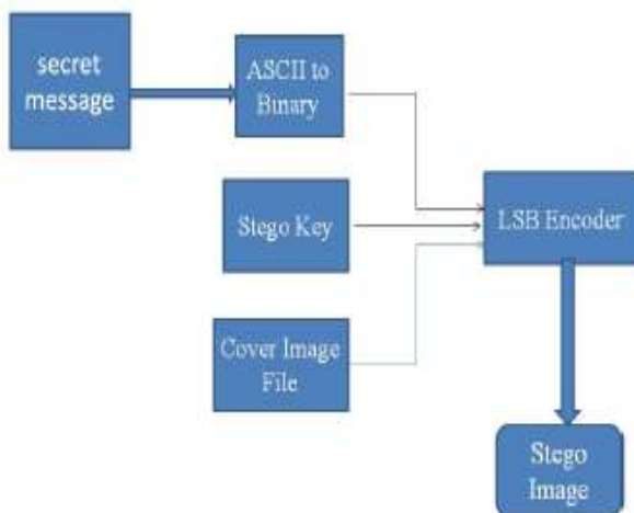
Figure 1: LSB insertion Mechanism
