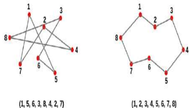
Figure 1.1: A visualization of symmetric TSP. (a) a twisted bad route (b) the optimum route
