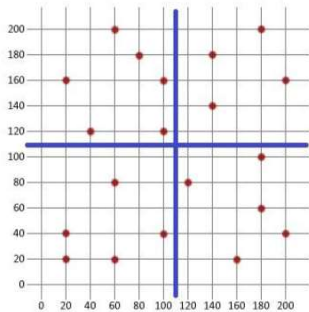
Figure 2: Map reduction
