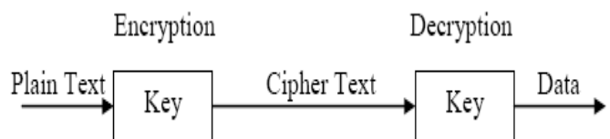
Figure 1: Cryptographic Model [2]
