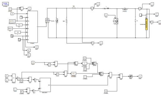
Fig:9. Simulation diagram of proposed system
