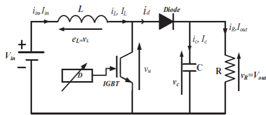
Fig:4. Circuit diagram of the Boost converter.
