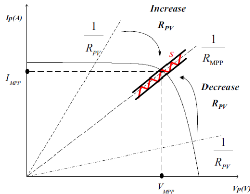
Fig.7-IV characteristics and MPPT process
