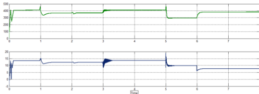
Fig:15. PVG power and Load feeding voltage
