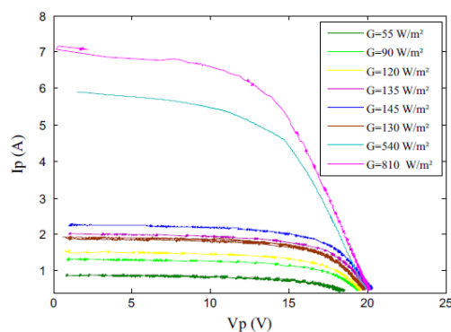
Fig: 3. I-V characteristics for different irradiances.
