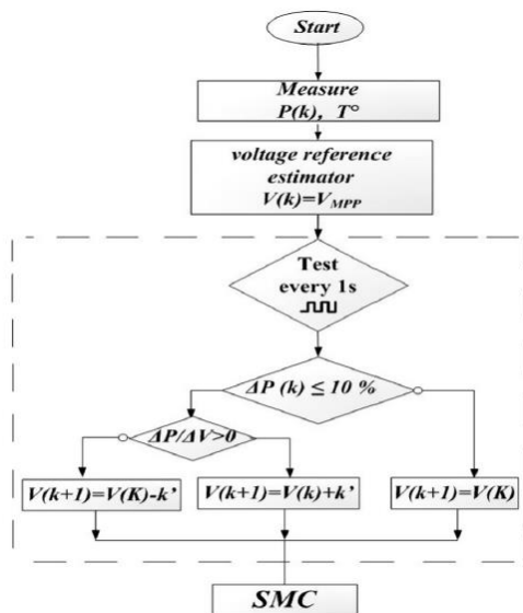
Fig:9.- PS-SMC algorithm flowchart
