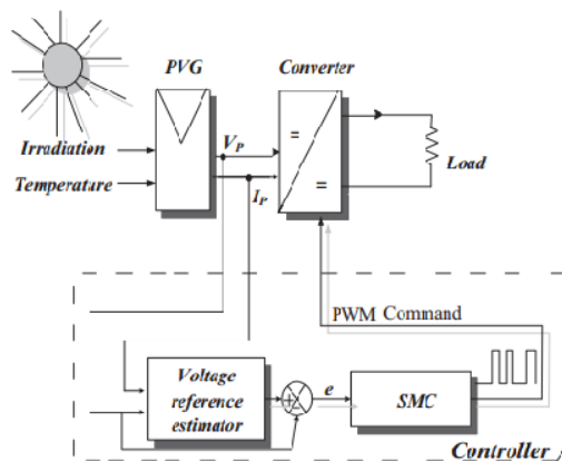
Fig:1. Synoptic diagram of PVG system
