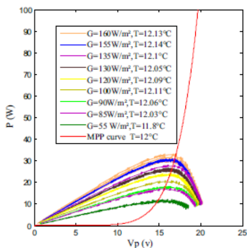
Fig:5. Real P-V characteristics for different irradiances at almost constant temperature.
