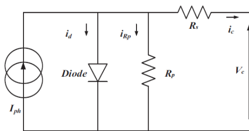
Fig.2 Equivalent circuit of PV cell
