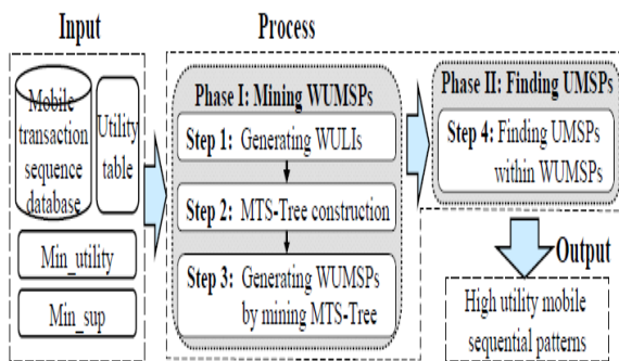
Fig. 1. The framework of the proposed algorithm UMSPDFG.
