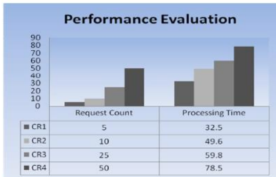
Fig 7: Performance Evaluation based on request count
