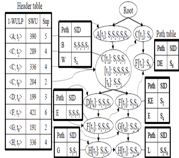
Fig. 3. An Example of MTS-Tree.
