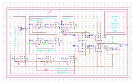
Fig 6: OpAmp with push pull amplifier
