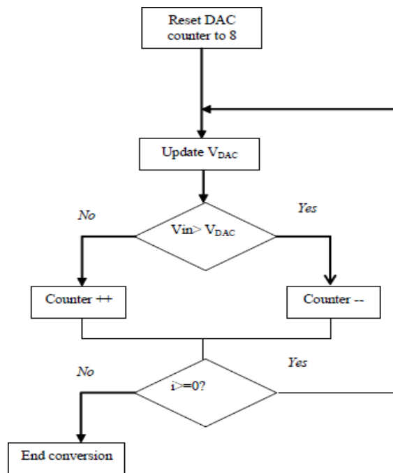
Fig 9: Algorithm of SAR ADC
