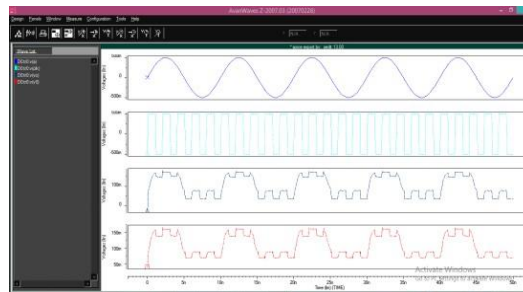
Fig 16: Output of S & H circuit
