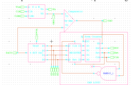
Fig 13: Schematic of SAR ADC 2
