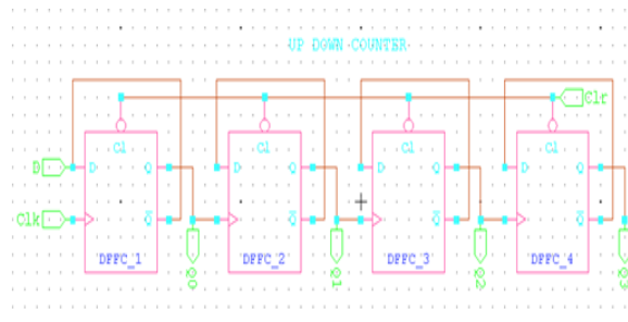
Fig 3: Schematic of 4 Bit counter
