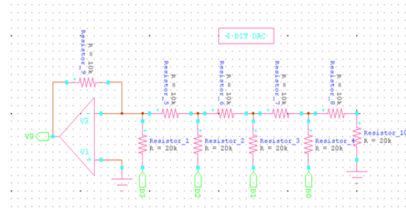
Fig 2: Schematic of D to A Convertor
