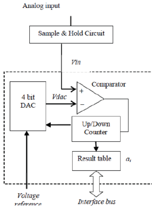
Fig 8: SAR ADC Circuit
