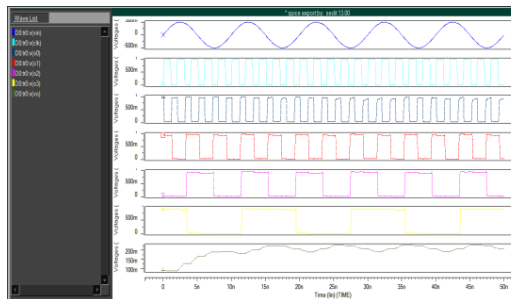
Fig 21: Output of SAR ADC 1
