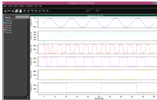
Fig 20: Output of SAR ADC 2
