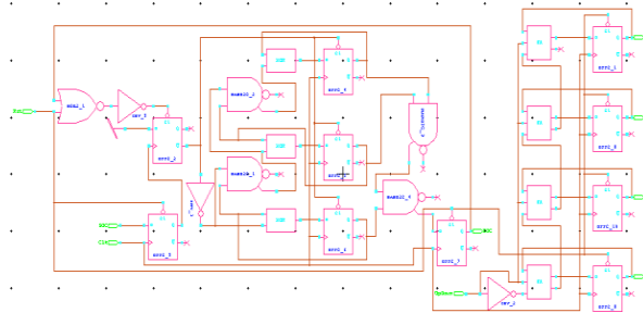
Fig 4: Schematic of Up Down Counter
