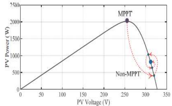
Fig. 4. P-V characteristics of the PV array. The dc-dc converter switches from MPPT to the Non-MPPT operation mode.
