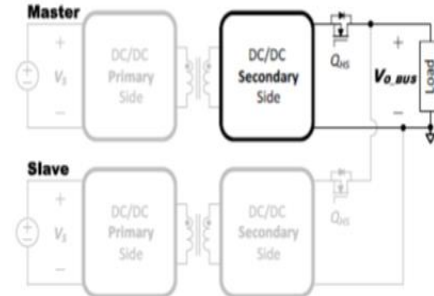
Fig. 4. Proposed circuit concept under a very light-load condition.
