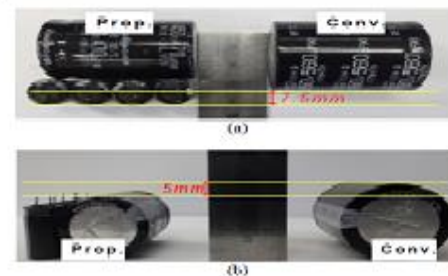
Fig. 7 Overall capacitor size. (a) Side view. (b) Top view.
