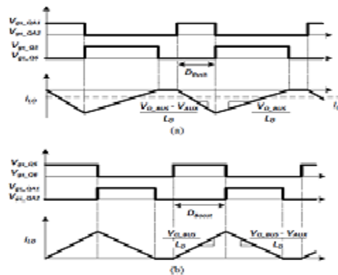
Fig. 9 Key waveforms of the bidirectional buck converter. (a) Discharging mode. (b) Charging mode.
