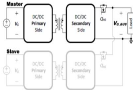
Fig. 3. CR concept under a light-load condition.
