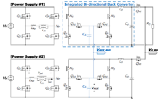
Fig 5. Circuit diagram of the proposed circuit
