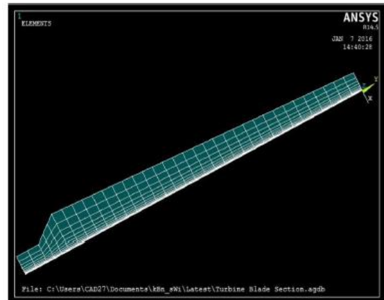
Fig. 4: Meshing
