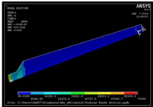
Fig. 6: Von-Mises Stress Distribution of Structural Steel
