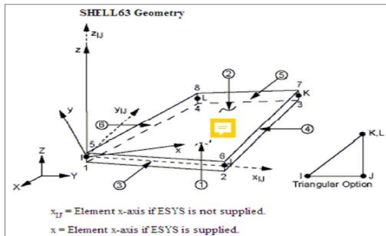
Figure 2 Shell 63 Element Geometry
