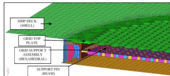
Figure 5 Details of the Finite Element mesh
