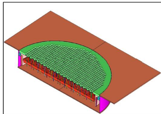
Figure 1 3D Half Cross-sectional view of grid assembly
