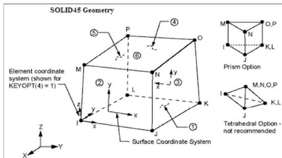
Figure 3 Solid 45 element geometry
