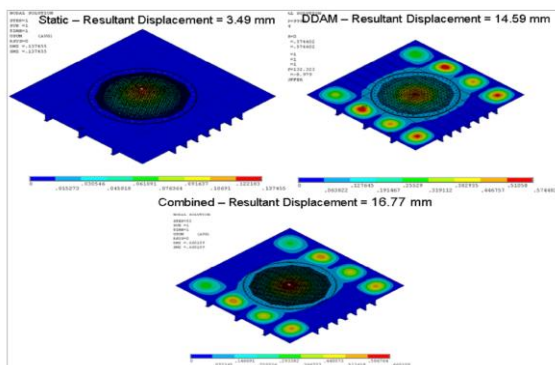
Figure 7 Total Displacement
