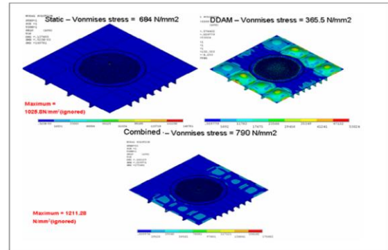
Figure 8 Total Vonmises stresses
