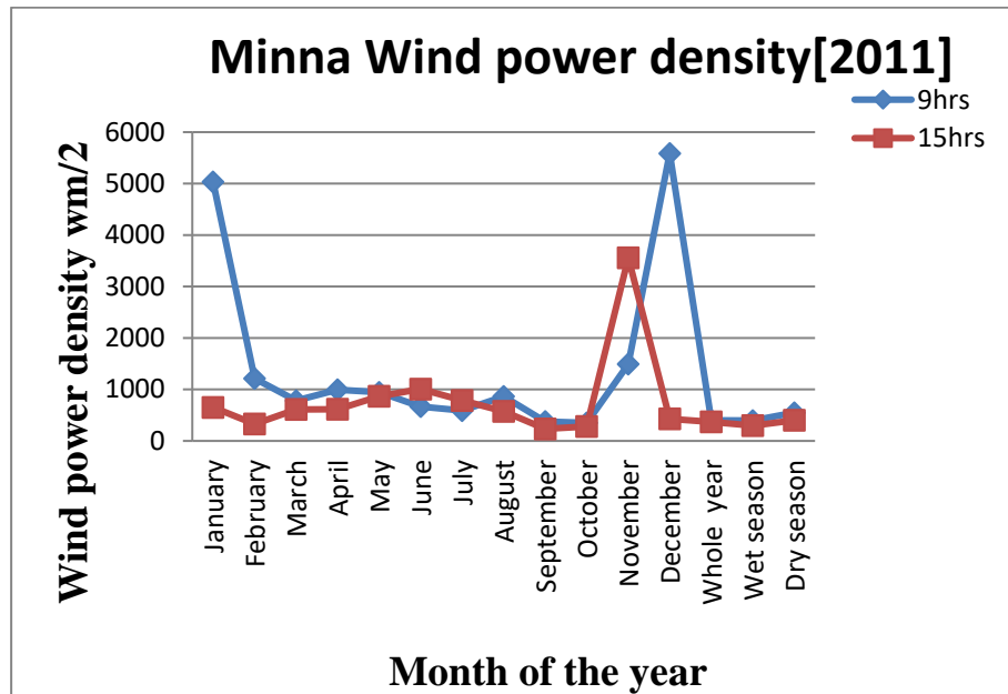
Figure 6; Minna Wind power density [W/m 2 ] versus month of the year.
