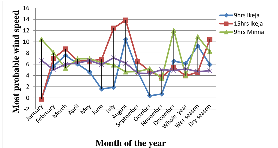
Figure 7; Mean monthly most probable wind speeds [ V_{mp} ] for Ikeja and Minna
