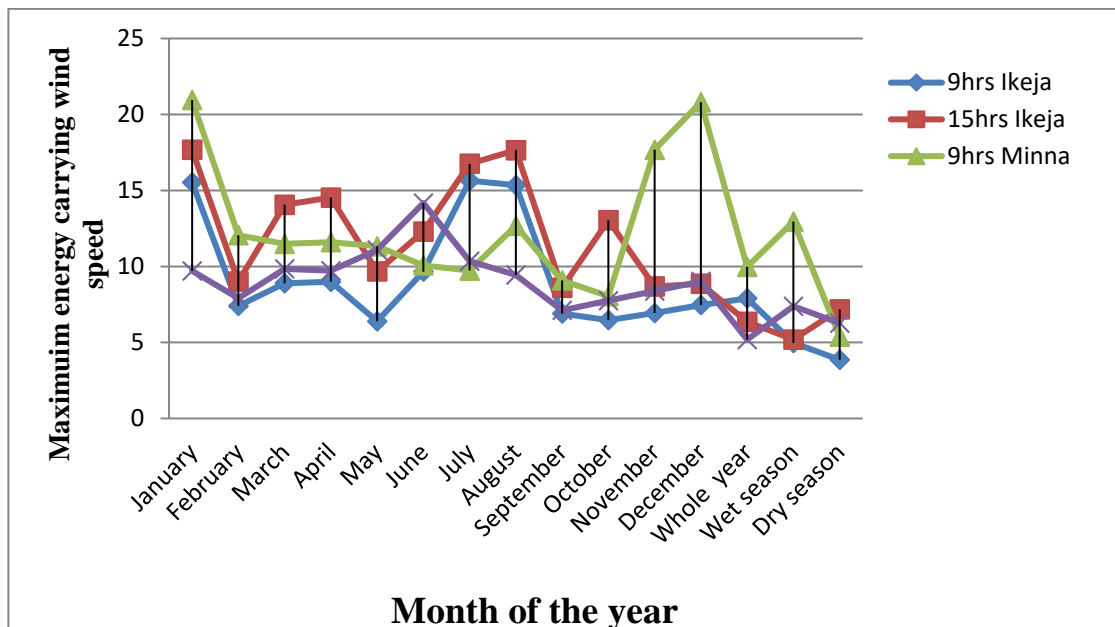
Figure 8; Mean monthly Maximum energy carrying wind speed [ V_{max} ] for Ikeja and Minna
