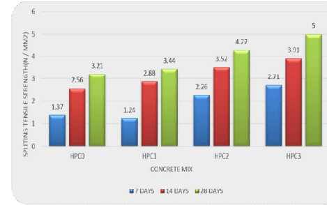
Chart -2: Split Tensile Strength Test Result
