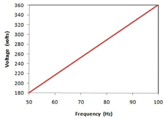
Figure 6 shows the variation of rotor voltage with its frequency of table II.
