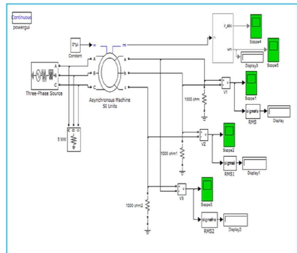
Figure 1. MATLAB Simulation diagram of MVFT
