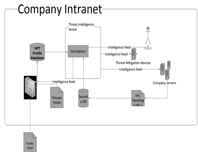
Figure 1: Proposed Threat Intelligence Architecture
