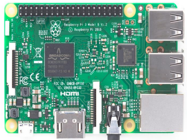
Fig 4.1:- Raspberry-Pi
