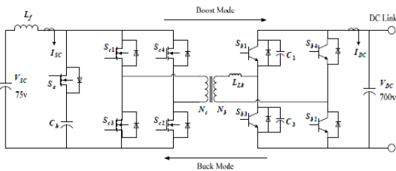
DC/DC converter structure
