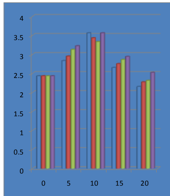
Fig 5.3 Split tensile Strength Vs % of combination of sodium polyacrylate and lime stone powder
