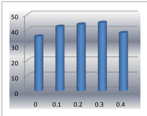
Fig 5.1 Compressive strength Vs % of cement replacement by Sodium polyacrylate Table 5.1 Compressive strength Vs % of cement replacement by Sodium polyacrylate
