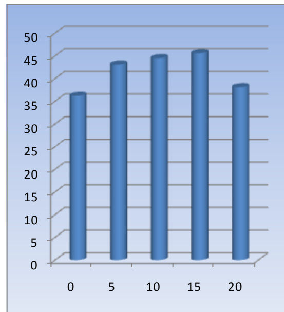
Fig 5.2 Compressive strength Vs % of cement replacement by Lime stone powder, Clinkers and Super plasticizer
