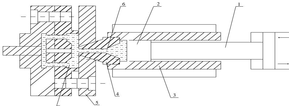
Figure 1. Scheme of equipment pouring details under pressure.
