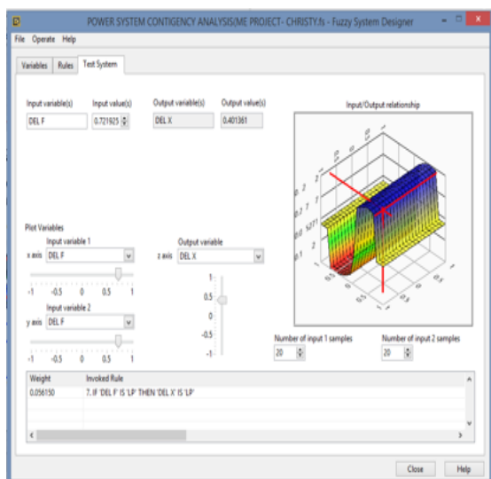
Fig. 4. Test system Input/ Output relationship.
