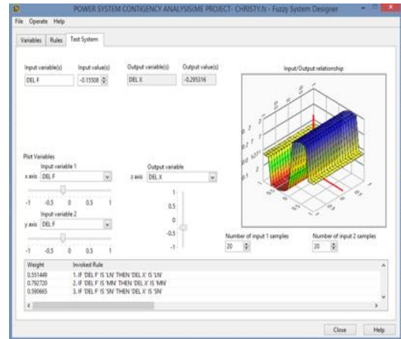
Fig. 5. Test system Input/ Output relationship.
