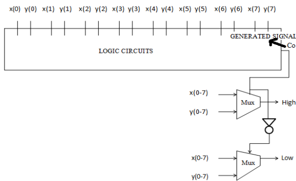
Fig. 1. Block Diagram of a Data Comparator
