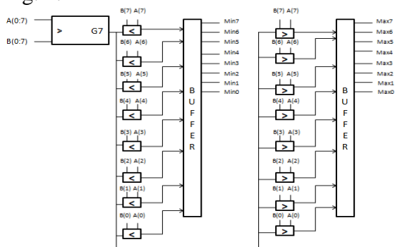
Fig. 2. Block Diagram of Conventional Data Comparator
