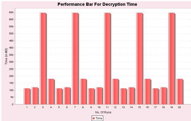
Figure 5 Decryption Time
