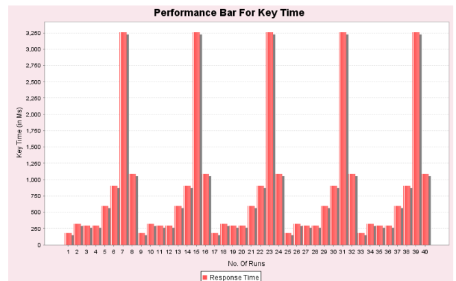
Figure 8 Key Generation Time
