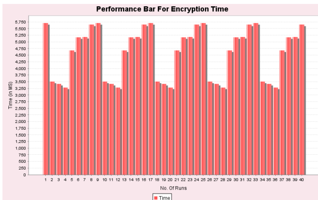
Figure 4 Encryption Time
