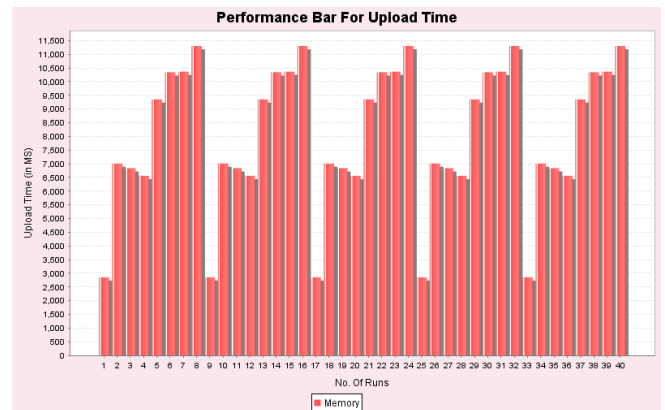
Figure 6 Upload Time
