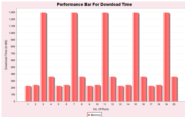
Figure 7 Download Time
