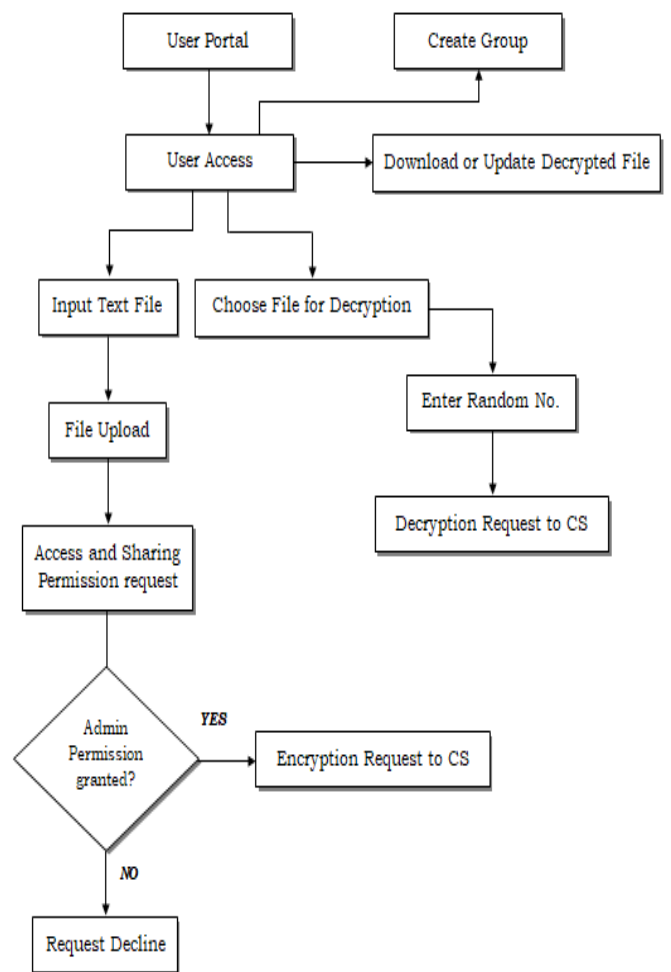
Figure 1 User Portal Activity
