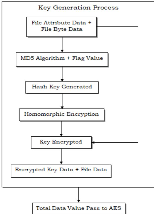
Figure 3 Key Generation Process
