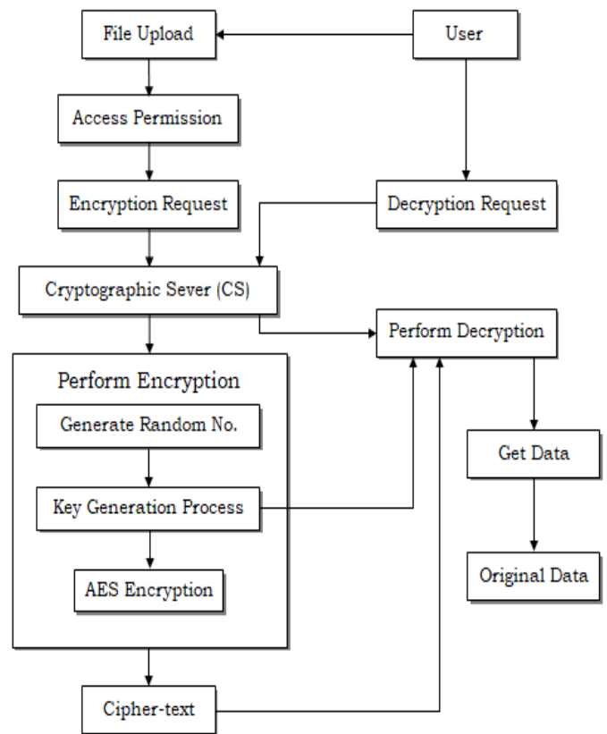
Figure 2 Cryptographic Working Process
