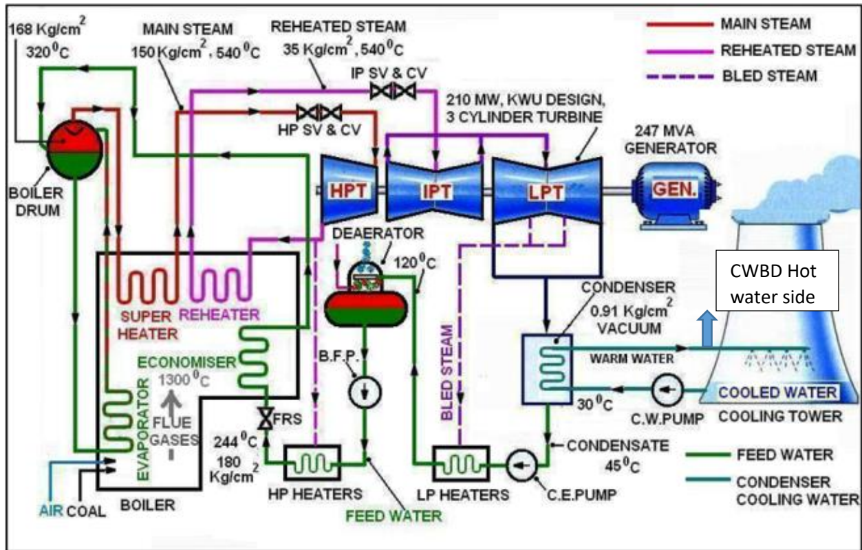
Fig-10A Modified scheme diagram of Thermal Power plant with WCT showing Hot CWBD
