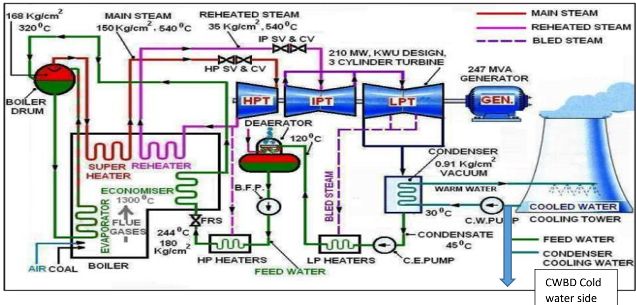
Fig-9 An Existing schematic diagram of Thermal Power plant with WCT.
