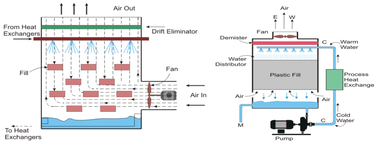
Fig-5 Forced Draft cooling tower [6] Fig-6 Forced Draft cooling tower [6]
